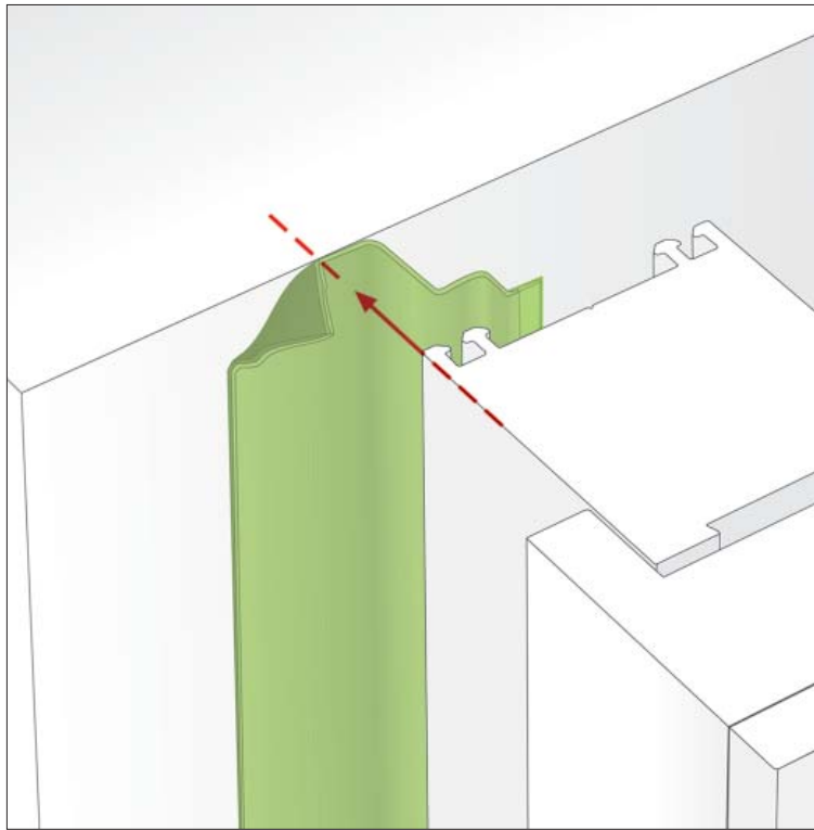
Figure 2 illbruck ME500 Duo "W" Flexible Window Membrane attachment
