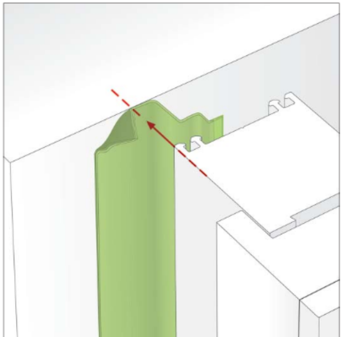
Figure 2 iLLBRUCK ME500 Duo 'W' Flexible Window Membrane attachment
