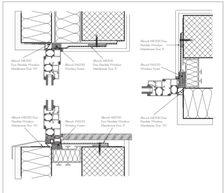
Figure 1 Typical installation details
