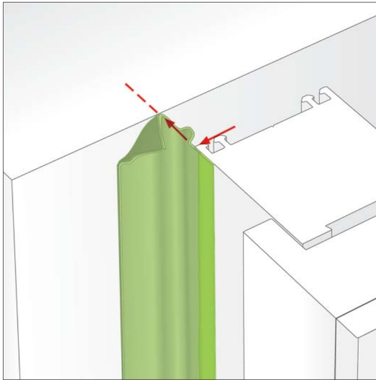
Figure 3 illbruck ME500 Duo 'E' Flexible Window Membrane attachment
