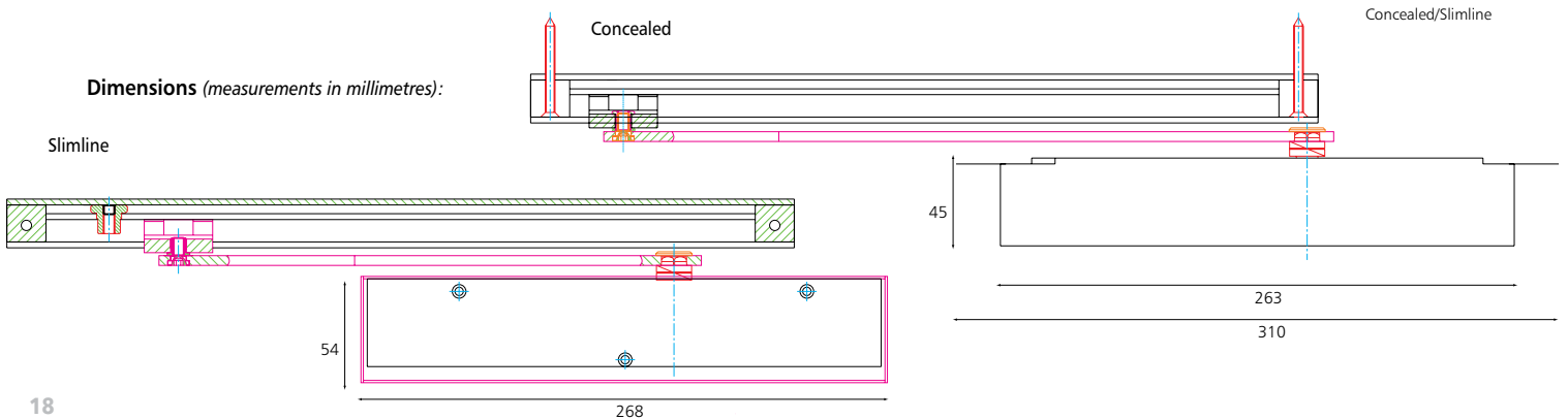
Concealed/Slimline
