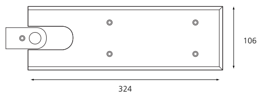
Cover plates
